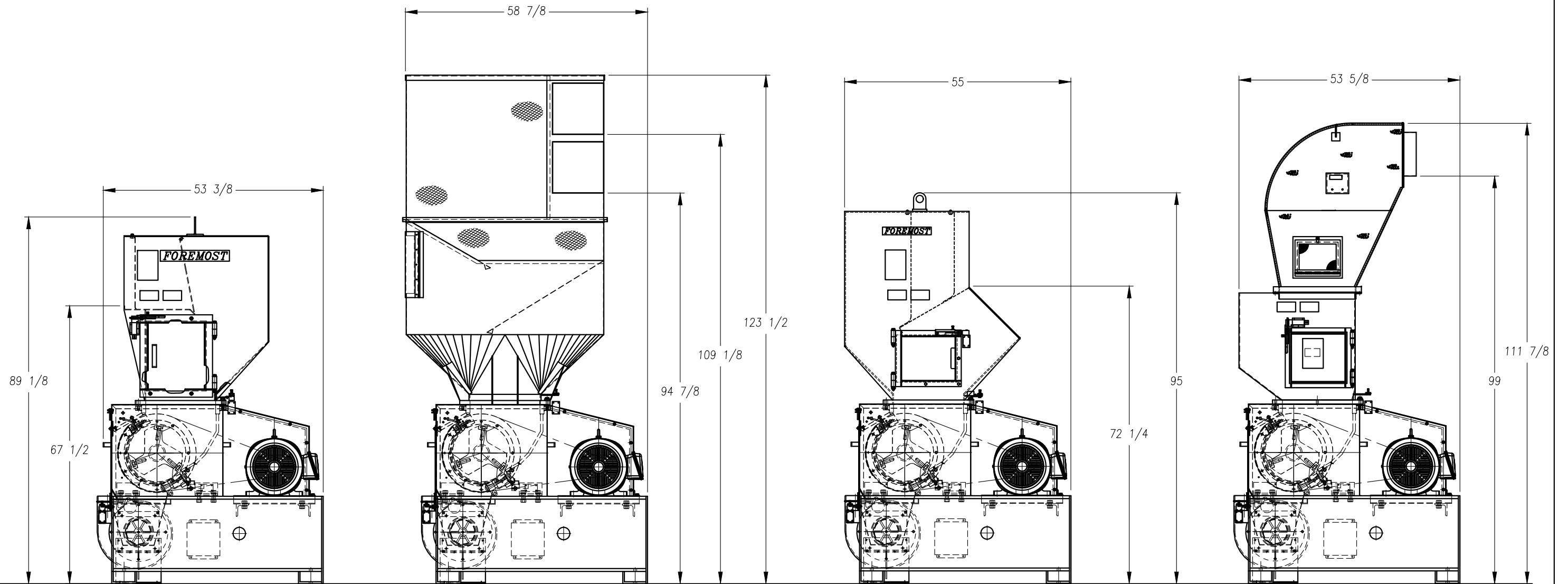
HD-5C GRINDER, W/ HANDFEED HOPPER & DB-5 BLOWER (REF W-7305-281)
